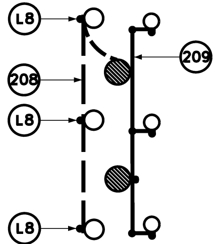
PLAN VIEW OF EARTH CONNECTION ON SEALING END PLATFORM
